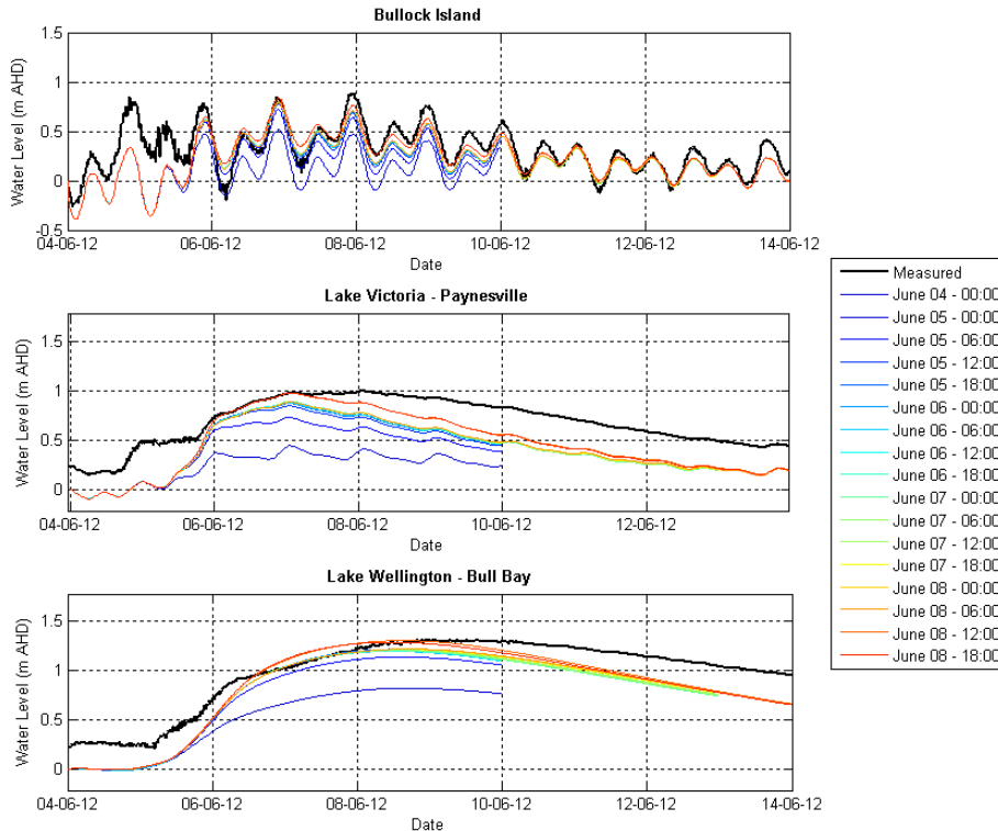
Figure 7 'Base Case' Lake Water Level Forecasts (June 2012 Event)
