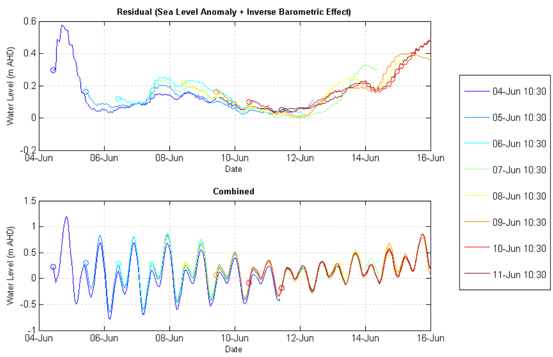
Figure 6 June 2012 Bureau OceanMaps SLA & Pressure Forecasts
