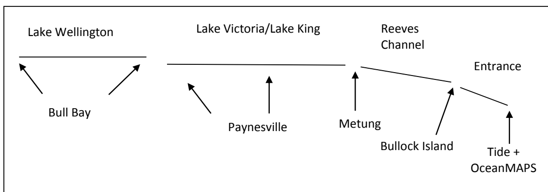
Figure 4: Schematic illustrating how initial water levels were defined throughout the Gippsland Lakes flood forecast simulations
