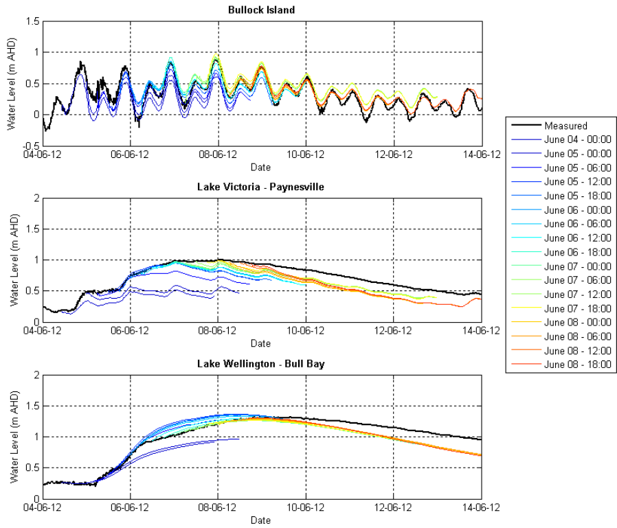
Figure 8 Real-time and Forecast Data Integration Lake Water Level Forecasts (June 2012 Event)
