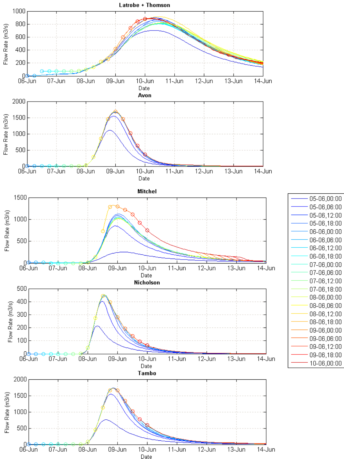
Figure 5 June 2012 Bureau URBS Streamflow Forecasts
