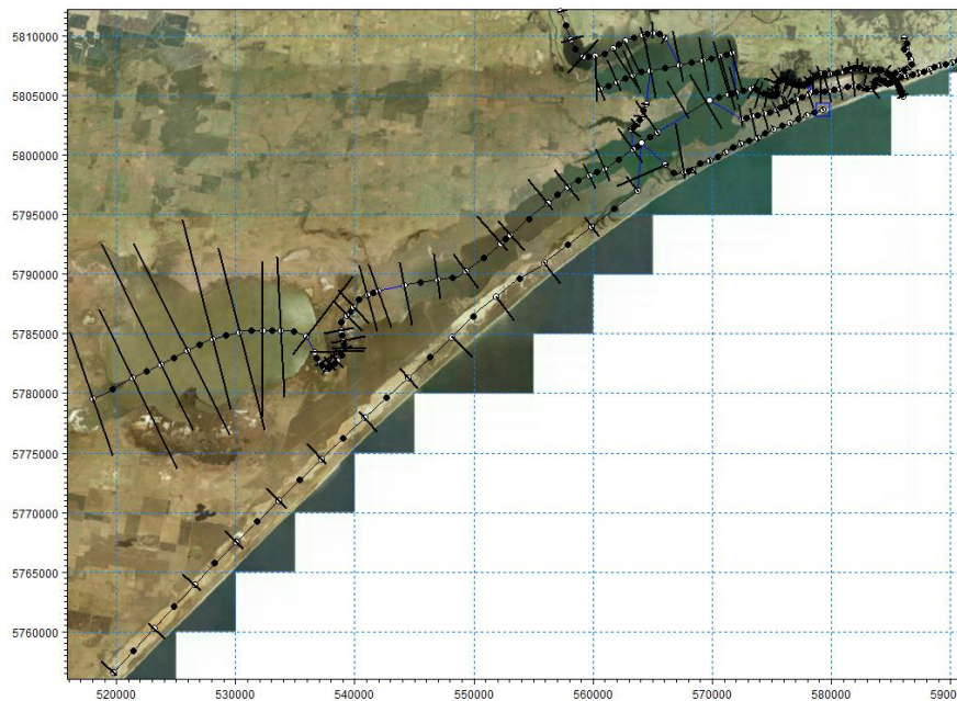
Figure 2 MIKE 11 Gippsland Lakes Cross Section Schematisation
