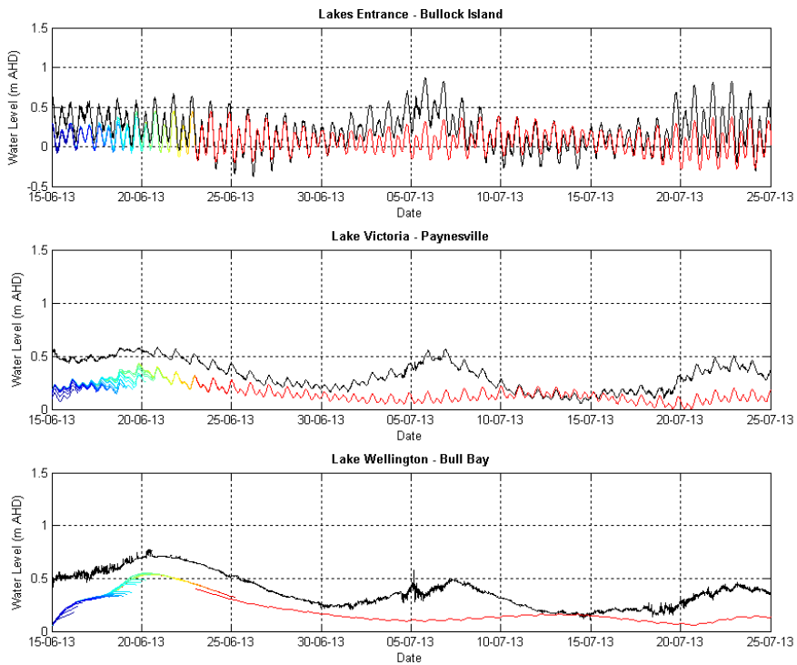
Figure 9 'Base Case' Forecast Comparisons to Measured Water Levels (June-July 2013 Event)
