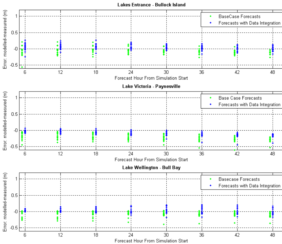
Figure 11 Absolute Forecast Error with Increasing Forecast Time for the June 2012 Flood Event
