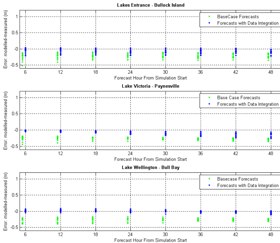
Figure 12 Absolute Forecast Error with Increasing Forecast Time for the June-July 2013 Event
