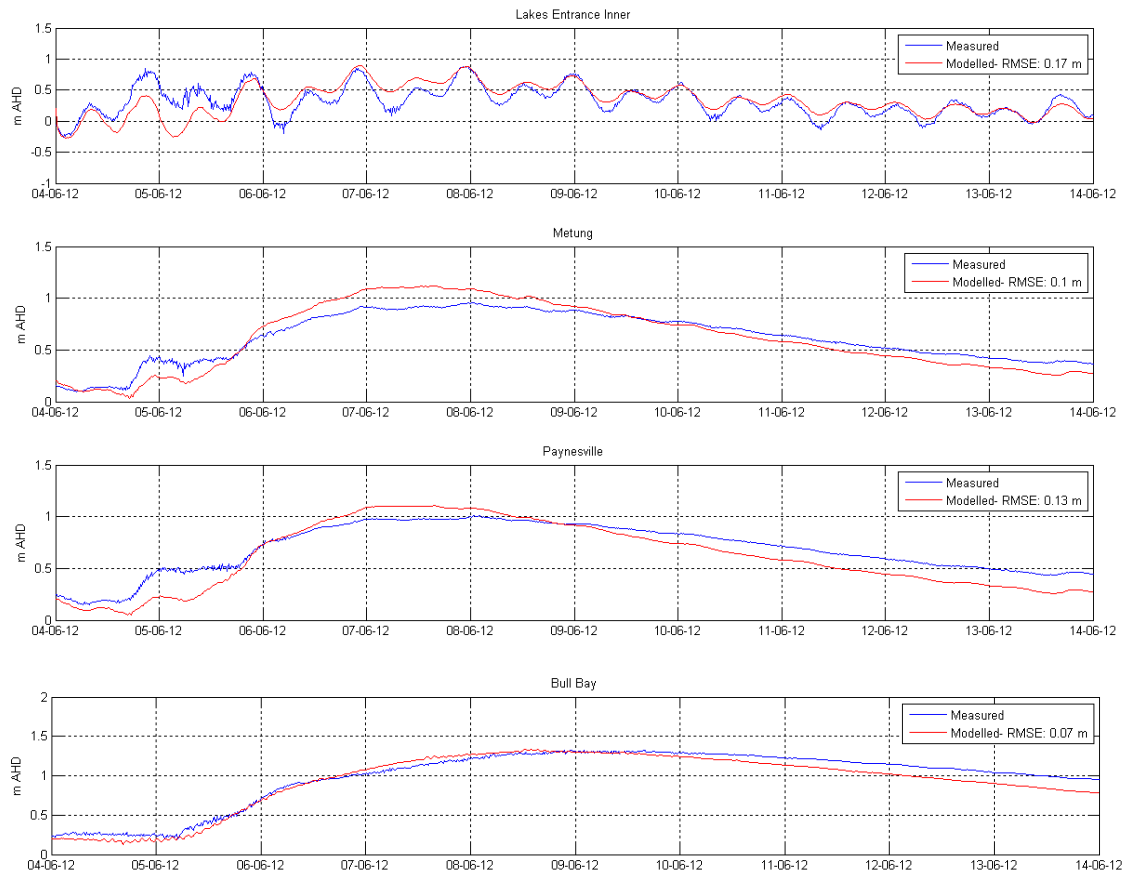
Figure 3 June 2012 Flood Event Calibration – Comparisons of Measured and Modelled Water Levels
