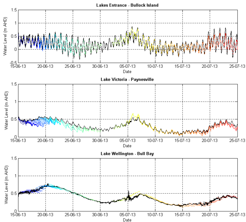
Figure 10 Real Time and Forecast Data Integration Forecast Comparisons to Measure Water Levels (June-July 2013 Event)
